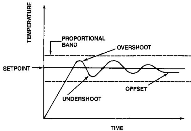
Fig. 10: Time Proportioning
