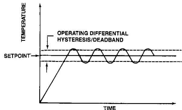
Fig. 9: On-Off
